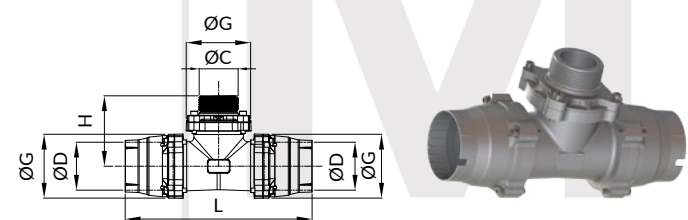
Reducing tee connection Connessione a Tee ridotta
