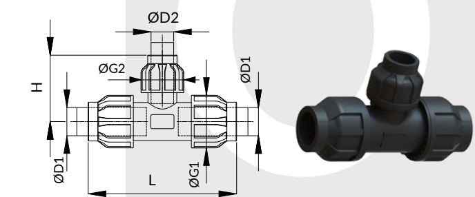
Reducing tee connection Connessione a Tee ridotta
