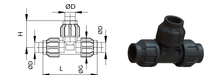
Tee connection Connessione a Tee
